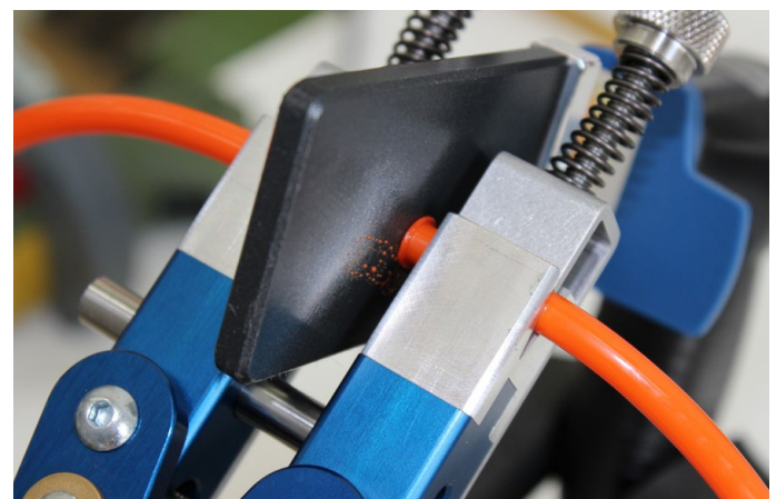
Paddle welding BEHAbelt EErgo with guide clamp FZ01 Vario
