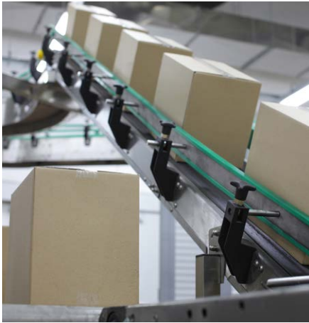
Belt conveyor
